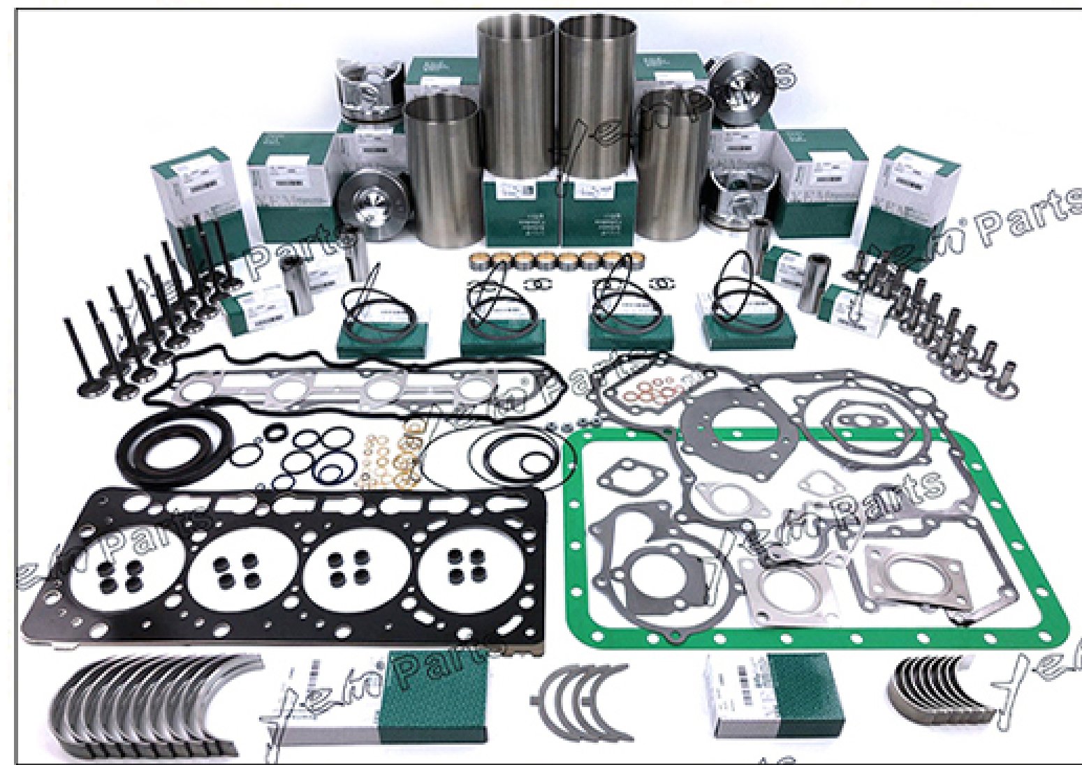
YEM-H8646 4TNV94组件
