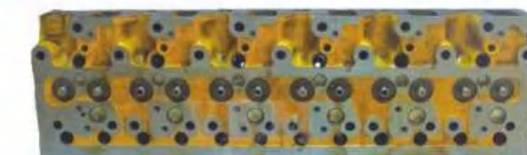
PC200-5 6D95缸盖 OEM: 6204-31-2203
