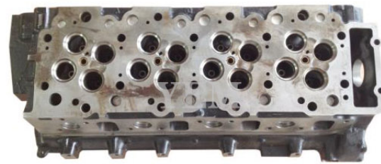
ISUZU 4HK1(1)
