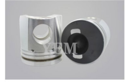
CUMMINS 6CT 3917707
